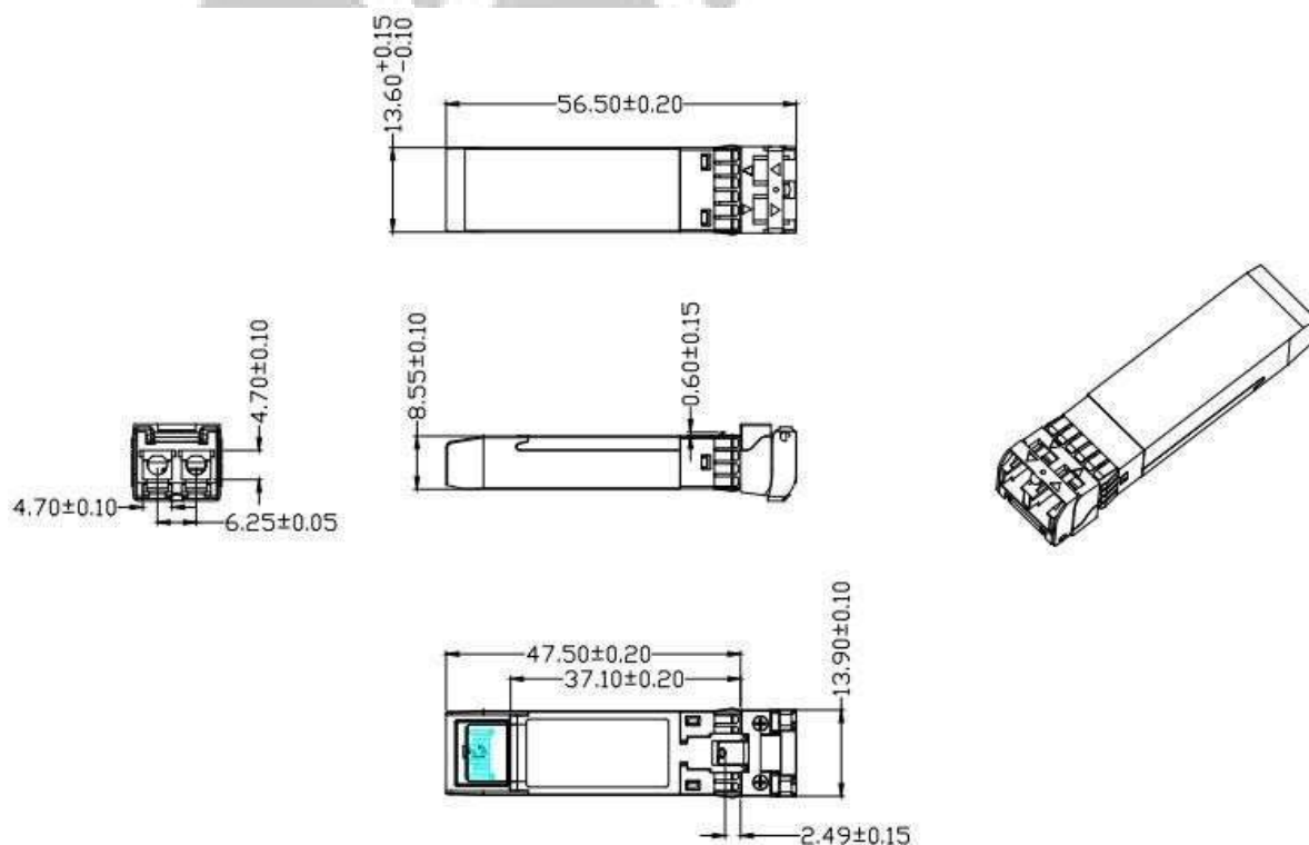
Figure5. Mechanical Specifications
