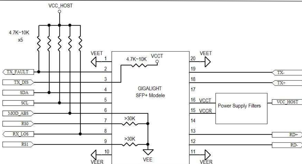
Figure4. Host-Module Interface
