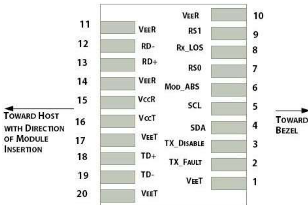
Figure 1: Interface to Host PCB
