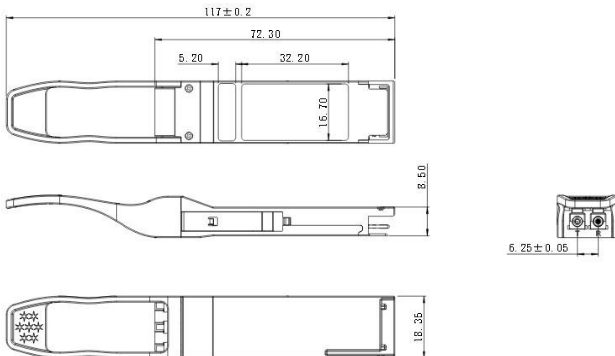
Figure 8. Mechanical Specifications
