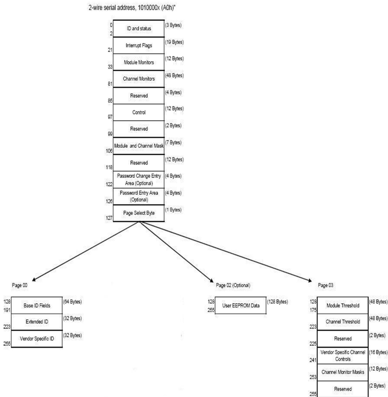
Figure5. QSF Memory Map
