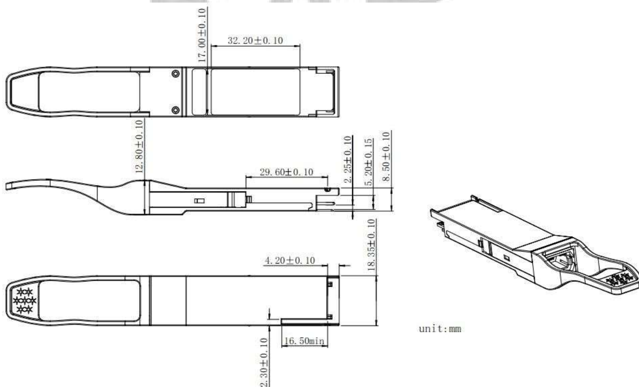
Figure10. Mechanical Specifications
