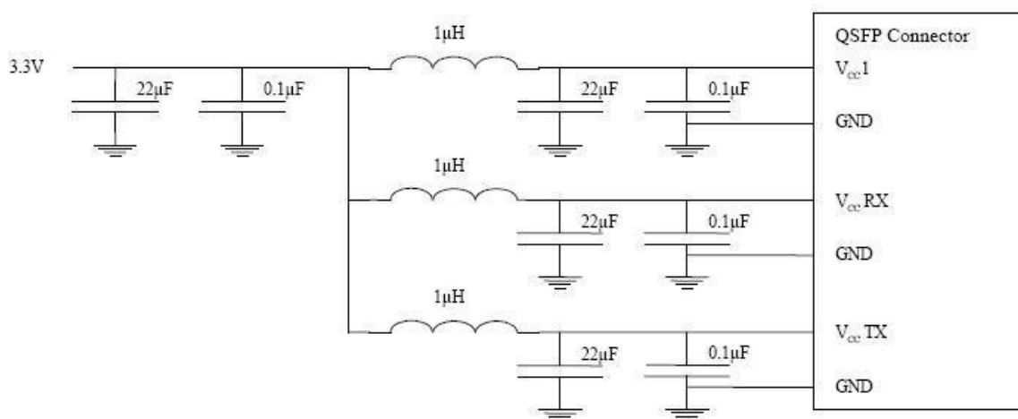
Figure3. Host Board Power Supply
